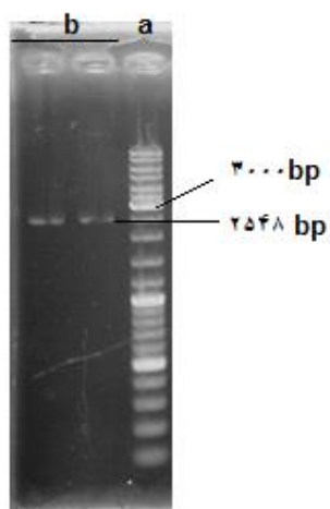
Fig3. Gel electrophoresis, pNZ8149( 2548bp)
