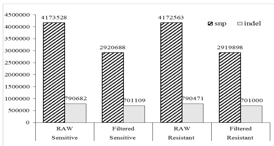
Fig1. Number of single nucleotide polymorphisms and small insertion-deletion before and after the filter.
