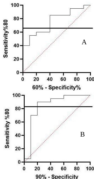
Fig 4. ROC curves of the studied genes in Asthenozoospermic and control subjects. A. ROC curve of ENTPD4 gene. B. ROC curve of IFT122 gene.
