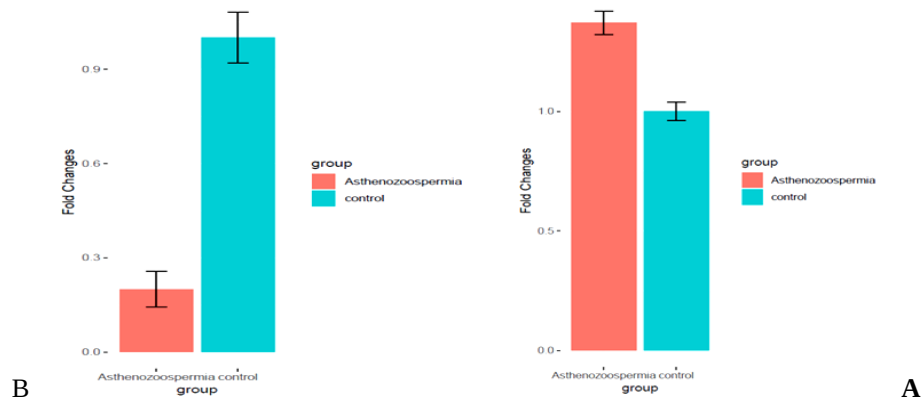
Fig 3. Gene expression alterations. A. The ENTPD4 gene expression pattern in patient and control group, B. The IFT122 gene expression pattern in patient and control group.
