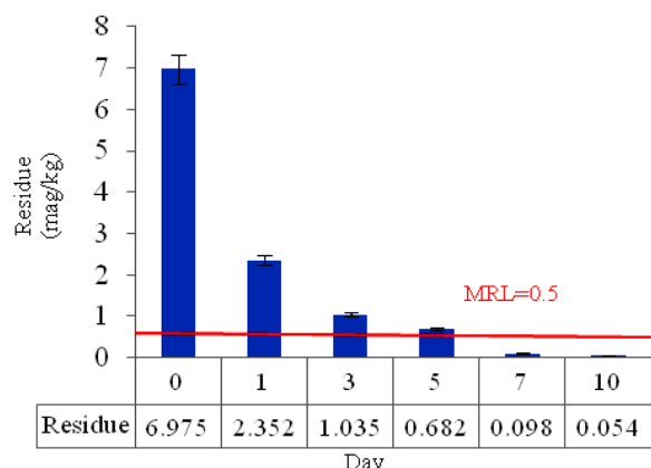
Fig. 4- The mean of Trans-Permethrin residues on different days in Tomato, Table 3- Mean Comparison of Trans-Permethrin residues with MRL (mg/ kg)
